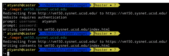
Figure 7. HTTP Basic Auth
